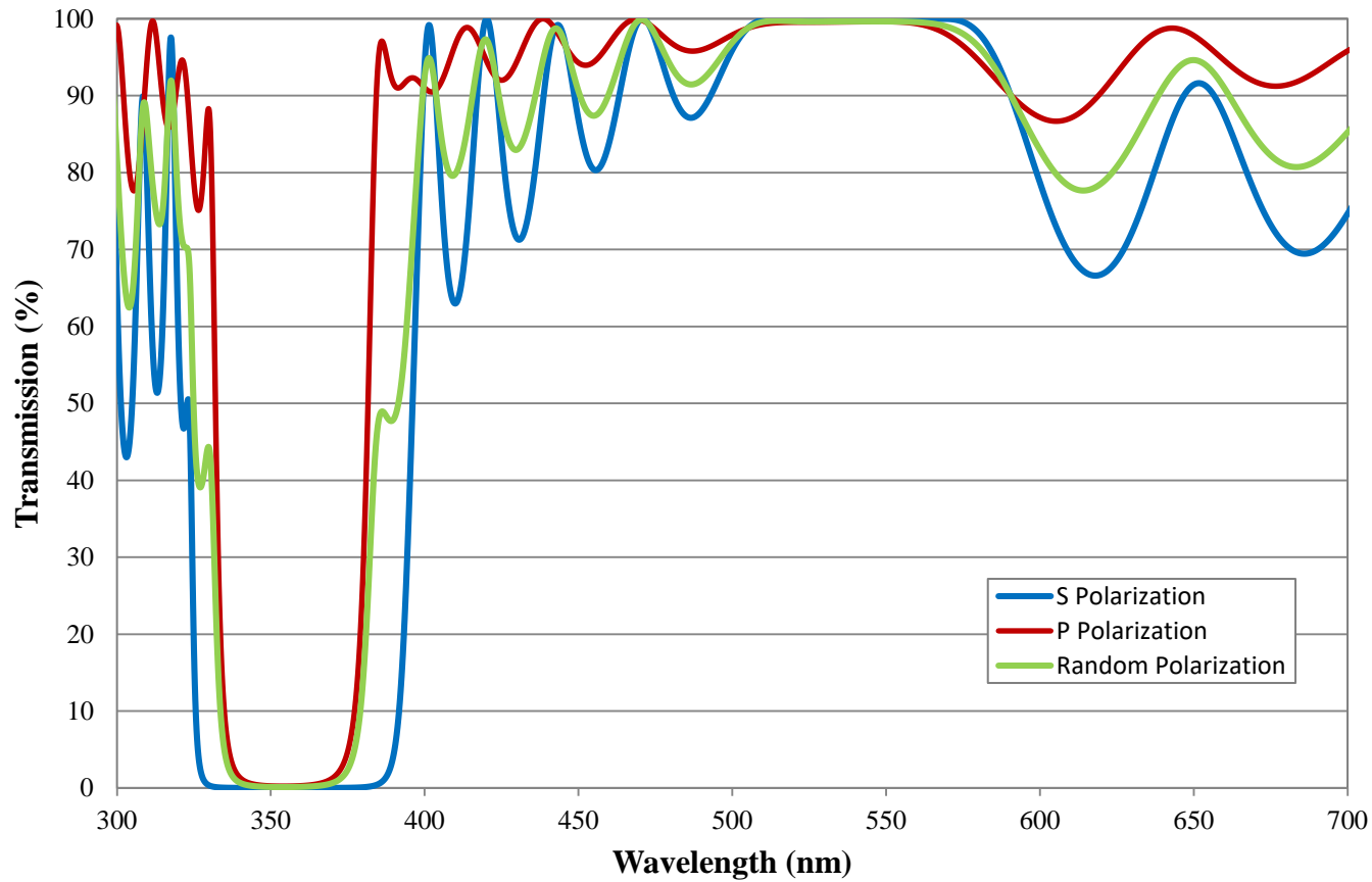
532nm T, 355nm R Harmonic Separator Typical Transmission FOR REFERENCE ONLY
