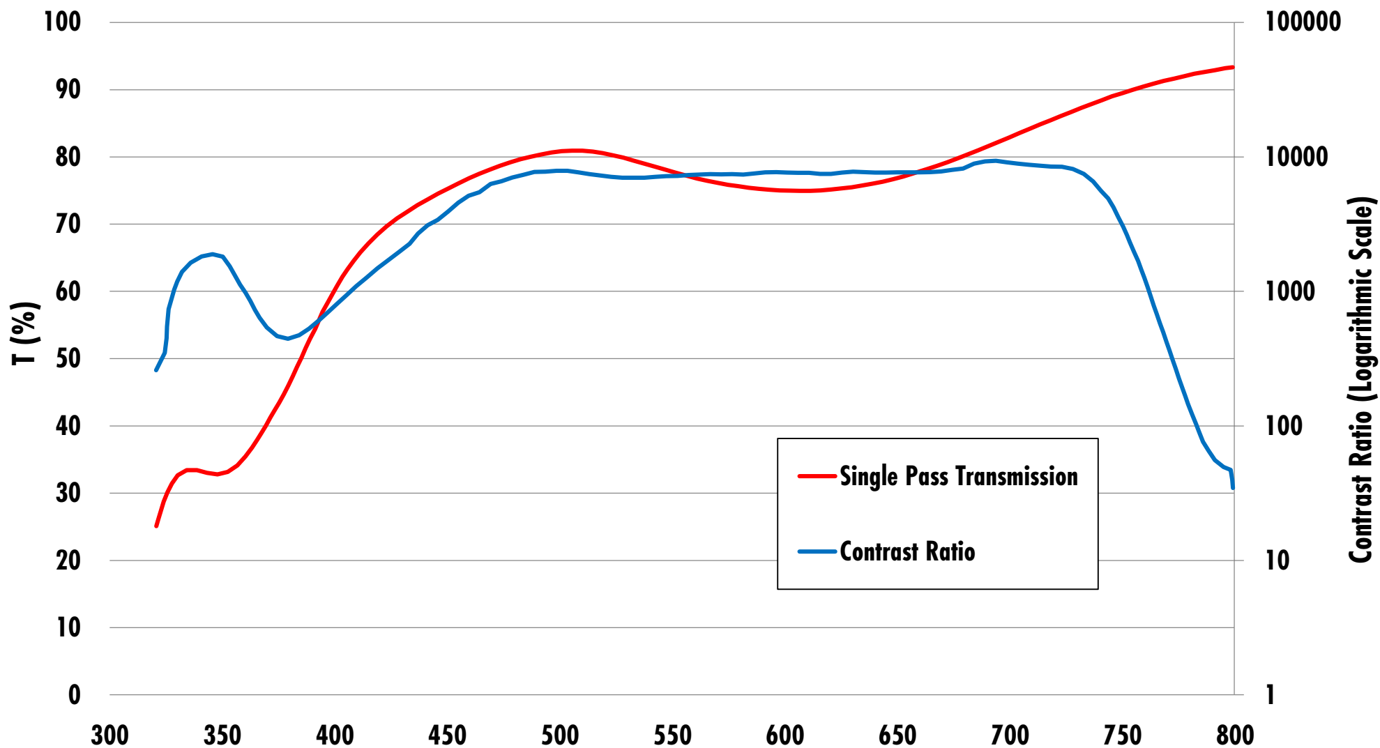
Ultraviolet (UV) Linear Polarizing Film Single Transmission and Contrast Ratio
